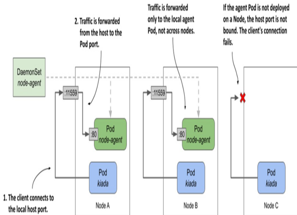
Figure 17.5 Exposing a daemon Pod via a host port
