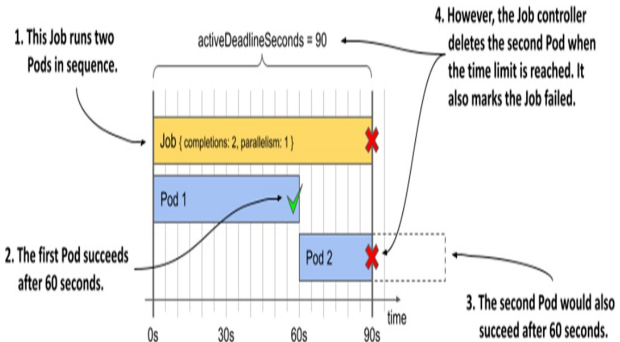
Figure 18.5 Setting a time limit for a Job
