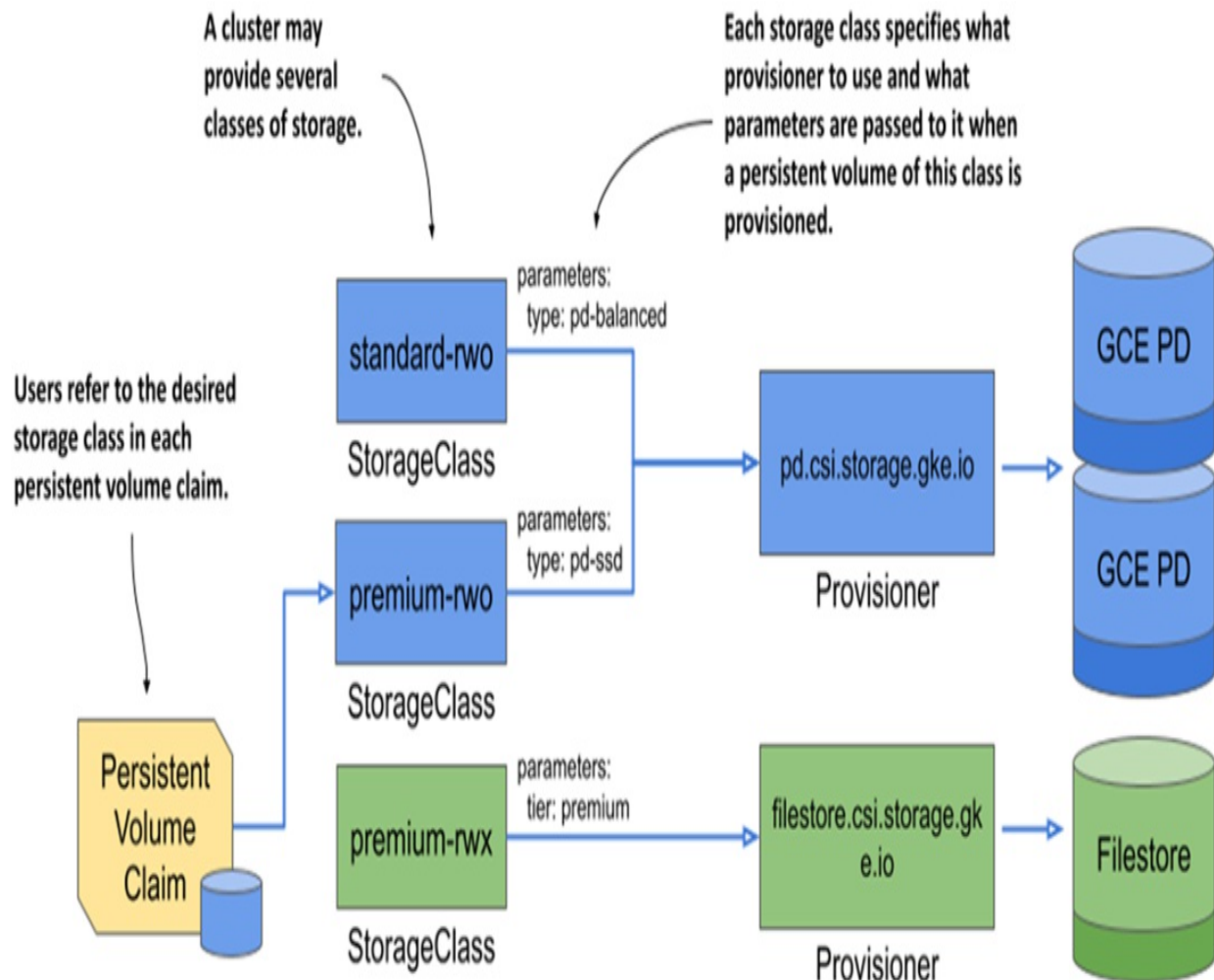
Figure 10.9 The relationship between StorageClasses, PersistentVolumeClaims and volume provisioners
