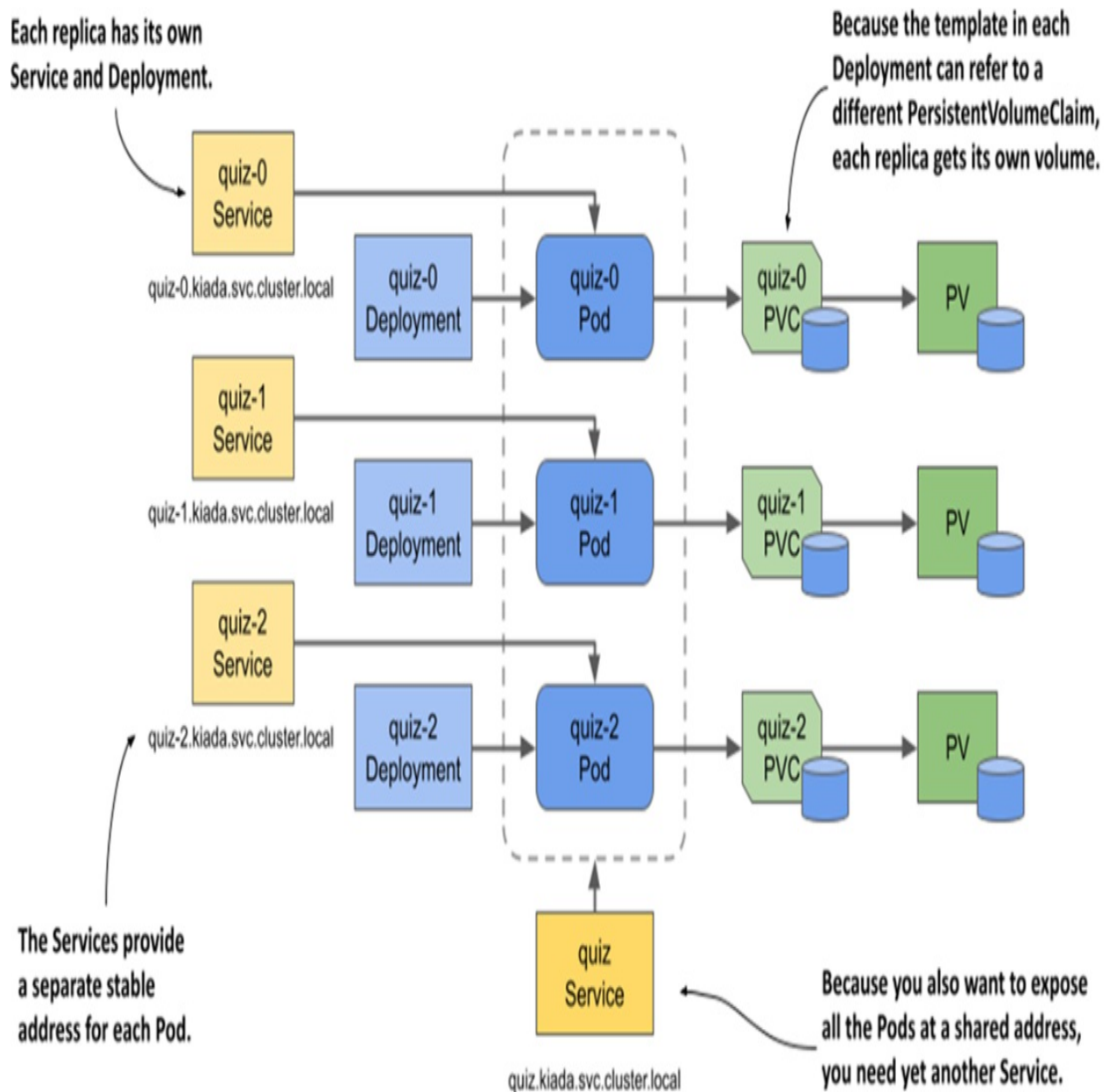
Figure 16.2 Providing each replica with its own volume and address.
