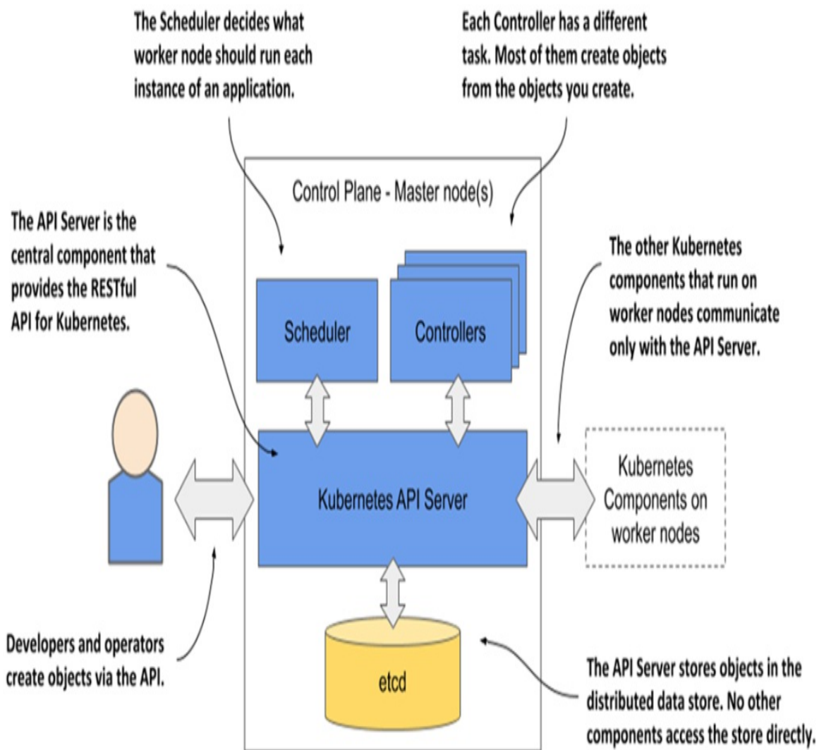
Figure 1.12 The components of the Kubernetes Control Plane
