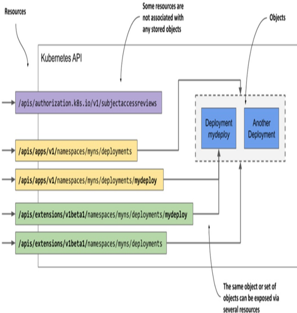
Figure 4.2 A single object can be exposed by two or more resources
