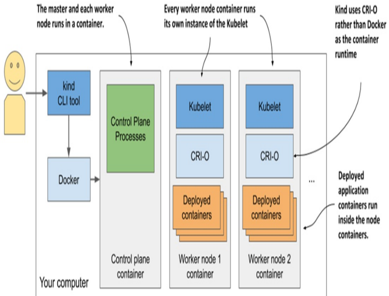
Figure 3.4 Running a multi-node Kubernetes cluster using kind
